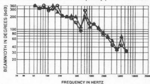
FIGURE 8 — DL12Sb Directivity vs. Frequency (TL12-1E enclosure)
