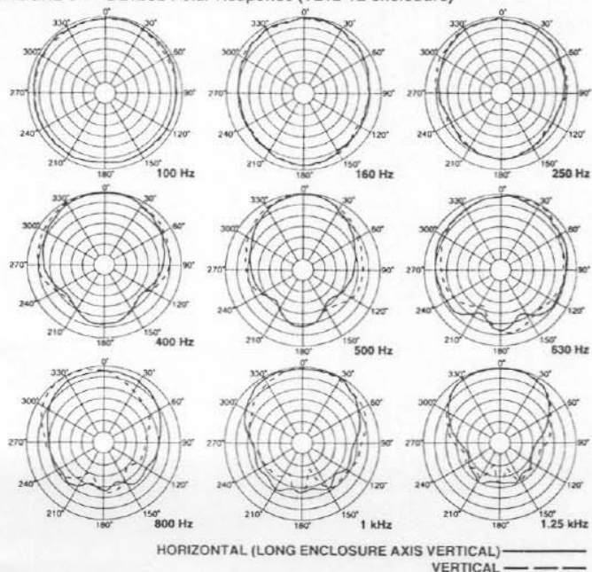
FIGURE 9 — DL12Sb Polar Response (TL12-1E enclosure)
