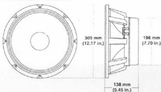
FIGURE 5 — DL12Sb Dimensions
